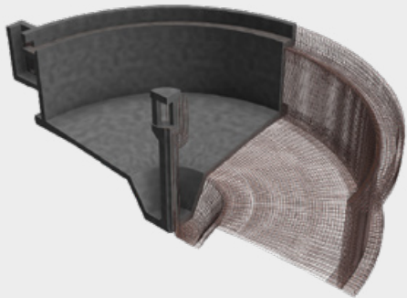
/ 3D REBAR
